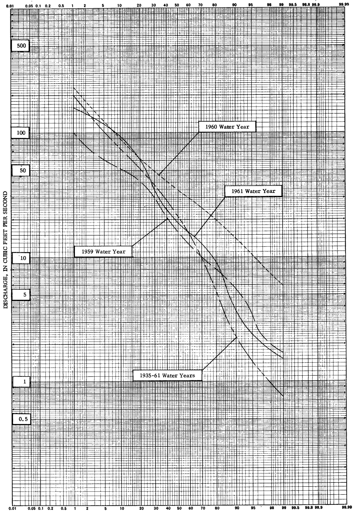
Figure 27. --Duration curves of daily flow, Ringwood Creek near Wanaque, N.J.
